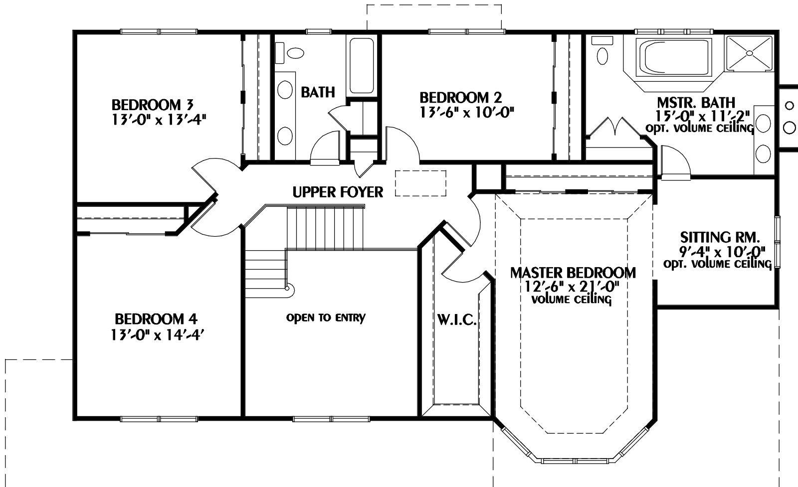
SECOND FLOOR PLAN LIVING AREA = 1,466 SQ.FT.
