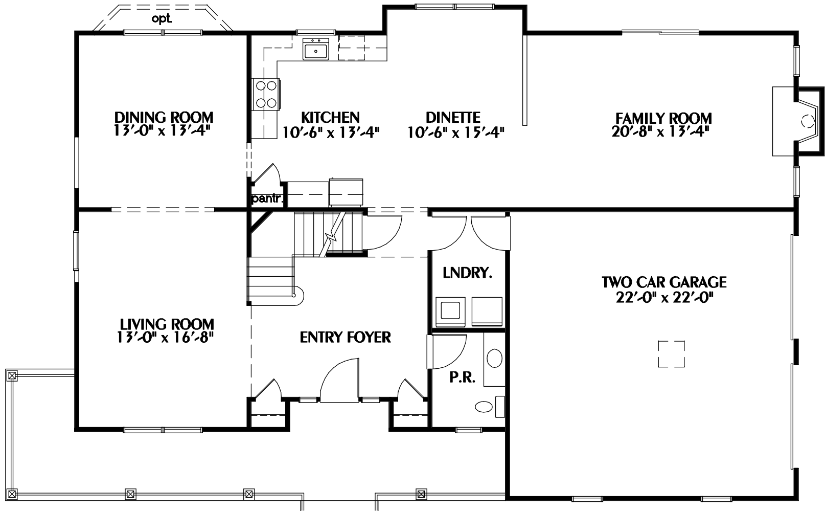
FIRST FLOOR PLAN LIVING AREA = 1,361 SQ.FT.
