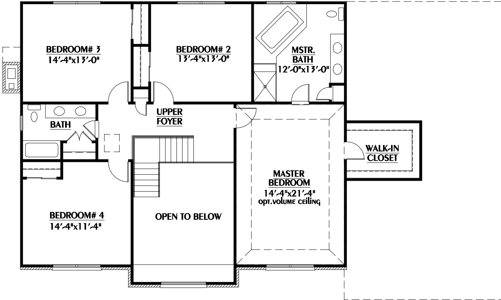
SECOND FLOOR PLAN LIVING AREA = 1,401 SQ.FT.
