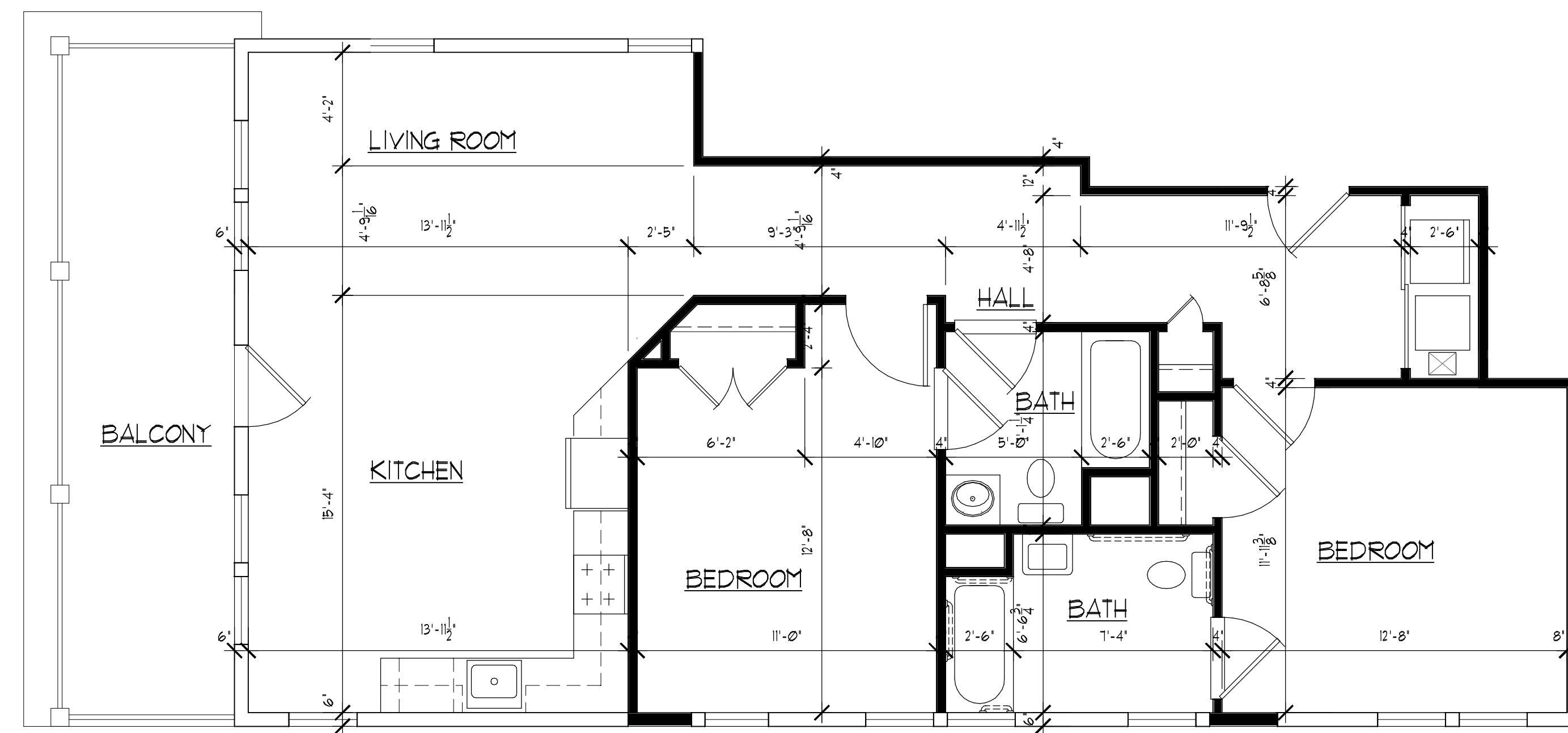
THIRD FLOOR PLAN UNIT 'F' SCALE 1/4" = 1'-0"
