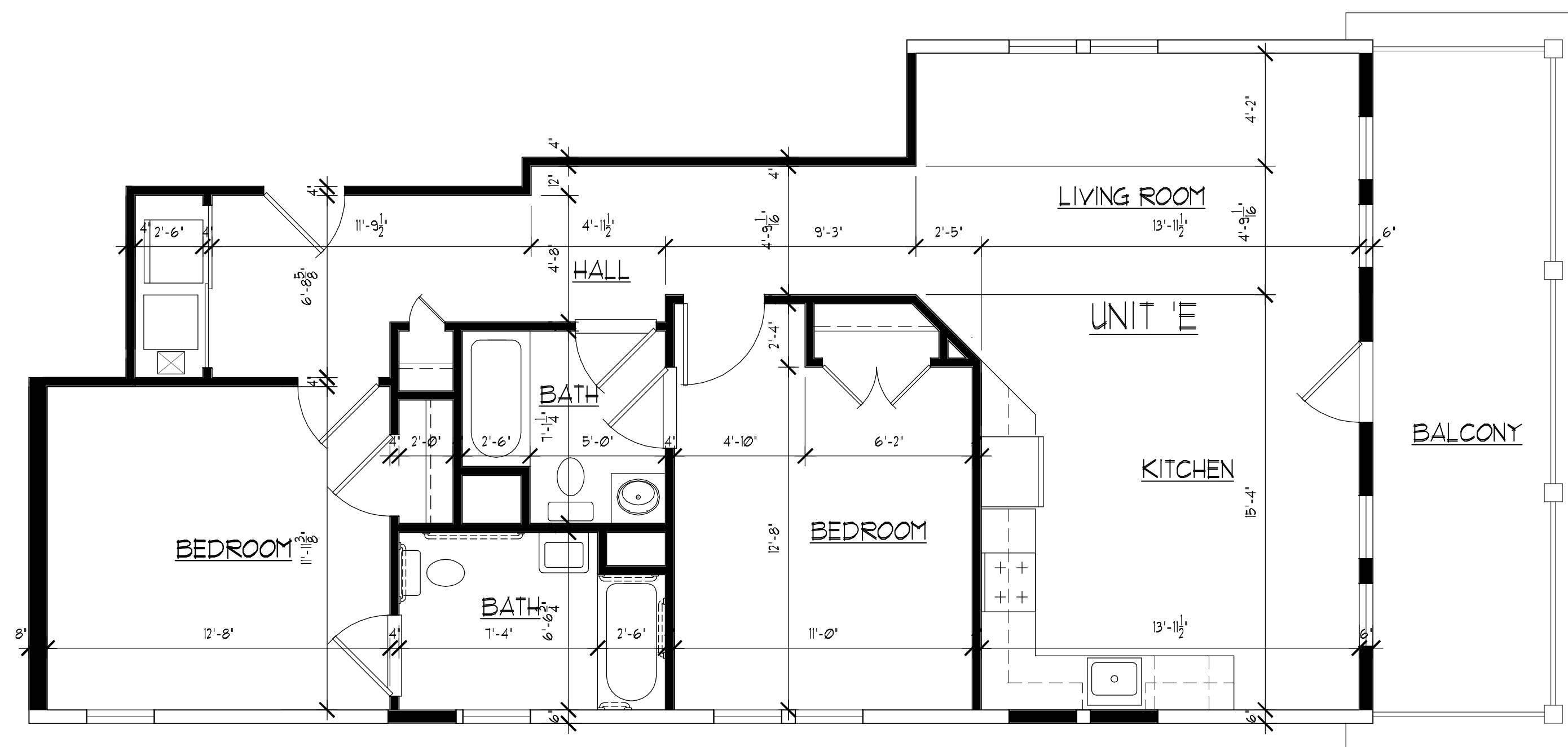
THIRD FLOOR PLAN UNIT 'E' SCALE 1/4" = 1'-0"
