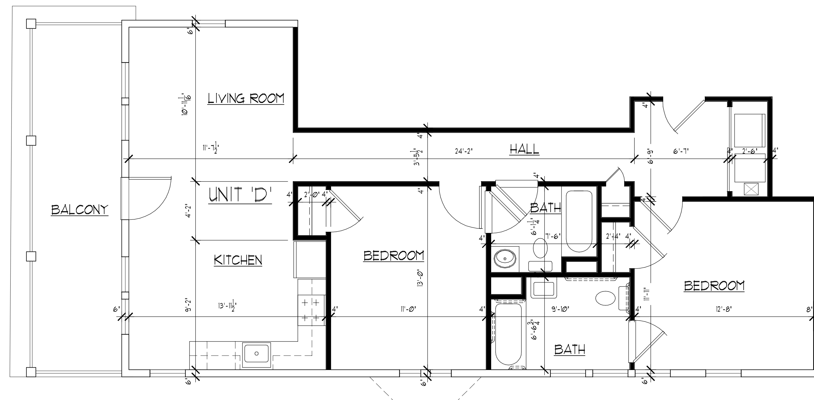
SECOND FLOOR PLAN UNIT 'D' SCALE 1/4" = 1'-0"
