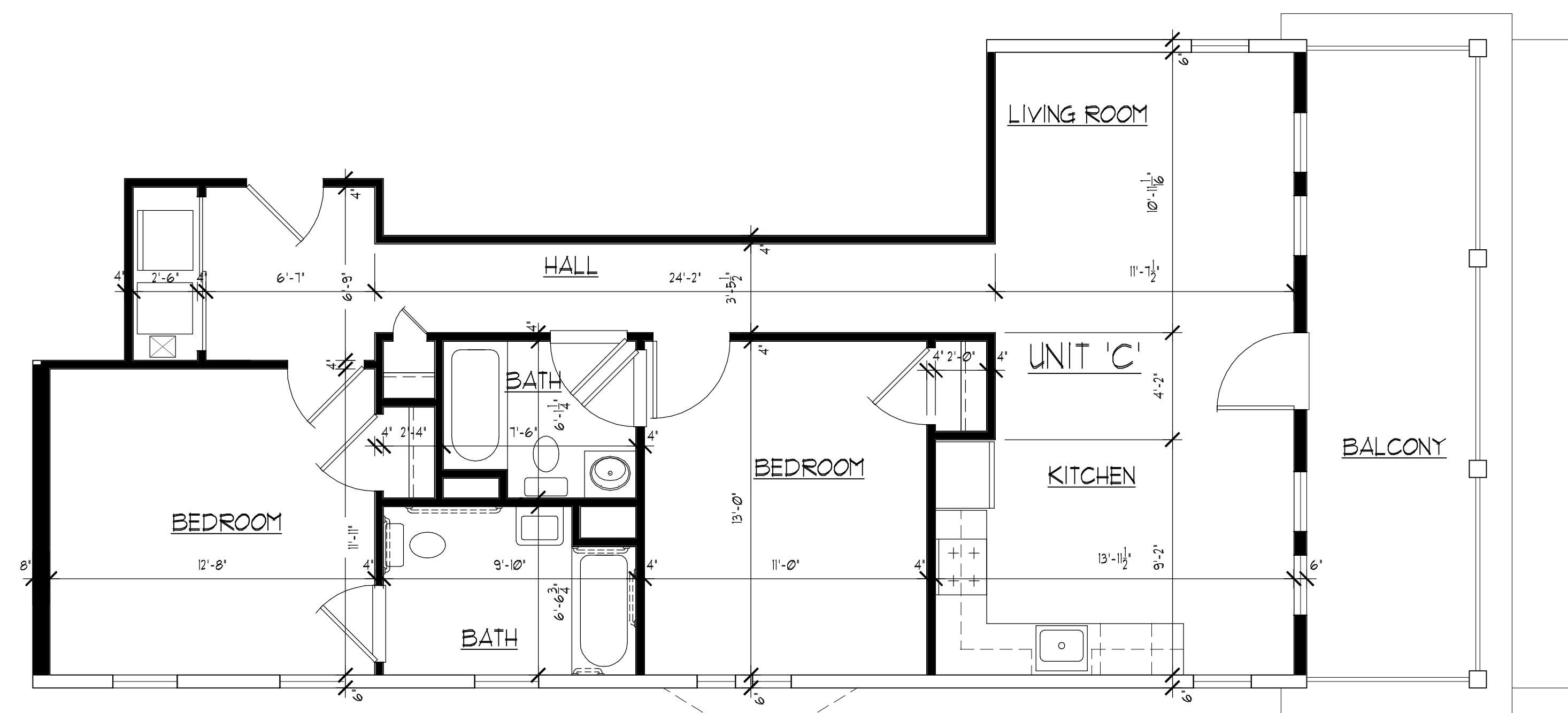
SECOND FLOOR PLAN UNIT 'C' SCALE: 1/4" = 1'-0"
