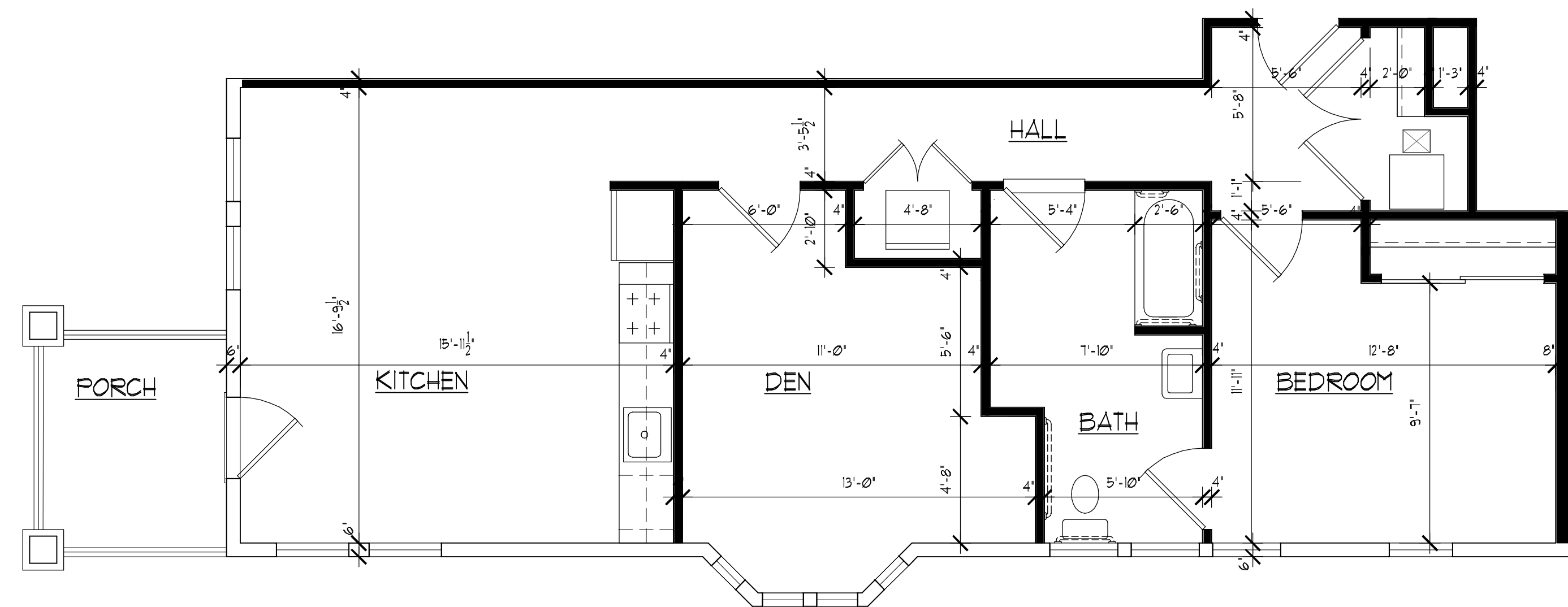
FIRST FLOOR PLAN UNIT 'B' SCALE 1/4" = 1'-0"
