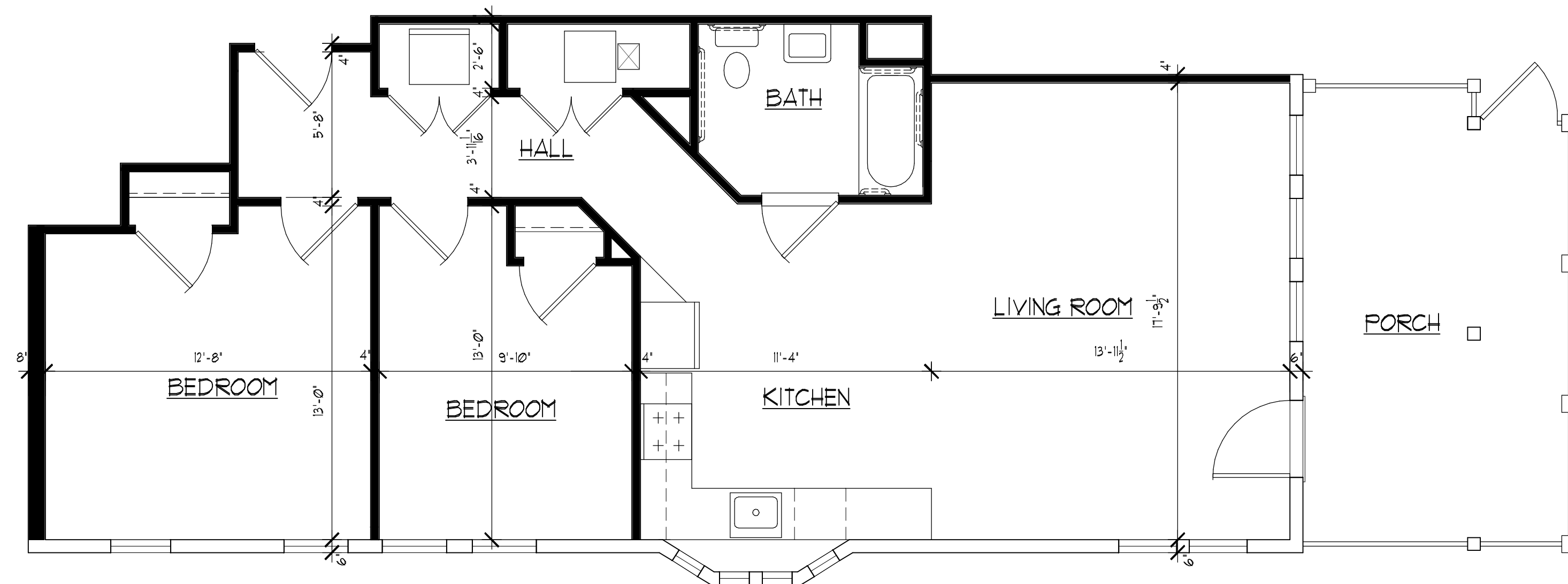
FIRST FLOOR PLAN UNIT 'A' SCALE 1/4" = 1'-0"
